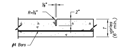
Contraction Joint
