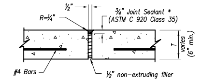
Expansion Joint
