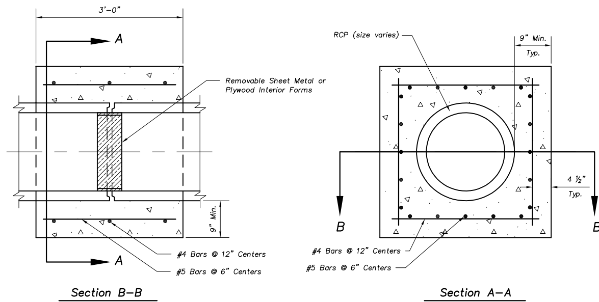
CONCRETE COLLAR DETAIL Not to Scale
